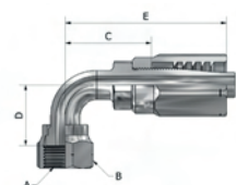
F O-Ring Seal Swivel
