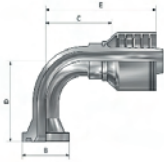
SAE Code 61 Flange
