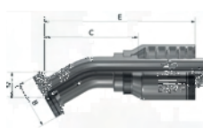
SAE Code 62 Flange
