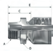
BSPT Male
