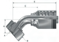
O-Ring Metric F 24° Cone
