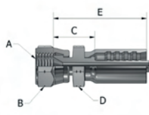
Komatsu F Swivel 30° Flare JIS Metric
