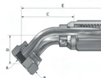
F O-Ring Seal Swivel
