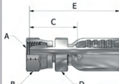
Metric F/M Ball Nose 24° Cone
