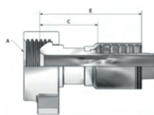
1502 Female Hammer Union
