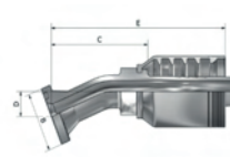
22.5 Degree
