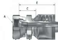
JIS (BSP) F Parallel Pipe Swivel
