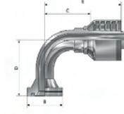
SAE Code 62 Flange
