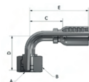
Metric Ball Nose F 24° Cone
