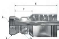
NPT F Swivel
