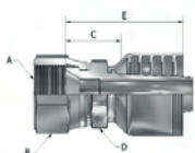
Komatsu F Swivel 30° Flare JIS Metric
