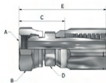
BSP F Parallel Pipe Swivel
