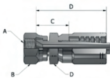
JIS (BSP) F Parallel Pipe Swivel
