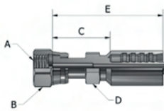
F O-Ring Face Seal Swivel
