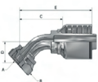
Ball Nose Metric F 24° Cone
