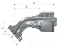
SAE Code 62 Flange
