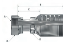
F O-Ring Face Seal Swivel
