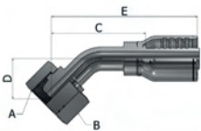
Ball Nose Metric F 24° Cone
